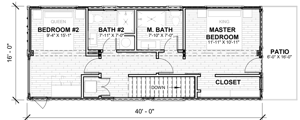
② LEVEL 2 MARKETING 1/8" = 1'-0"
