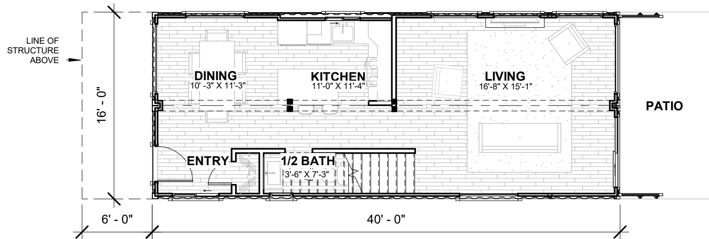
① LEVEL 1 MARKETING 1/8" = 1'-0"
