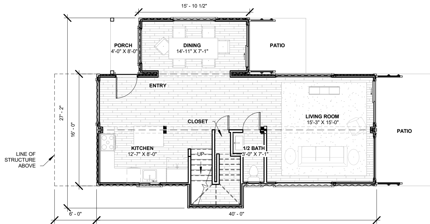
① LEVEL 1 1/8" = 1'-0"
