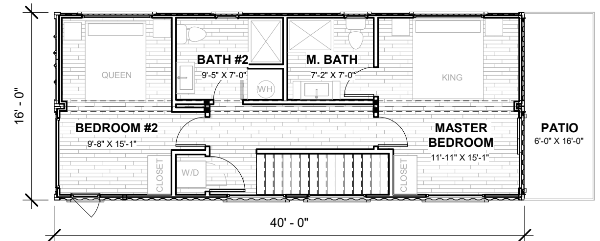
② LEVEL 2 1/8" = 1'-0"
