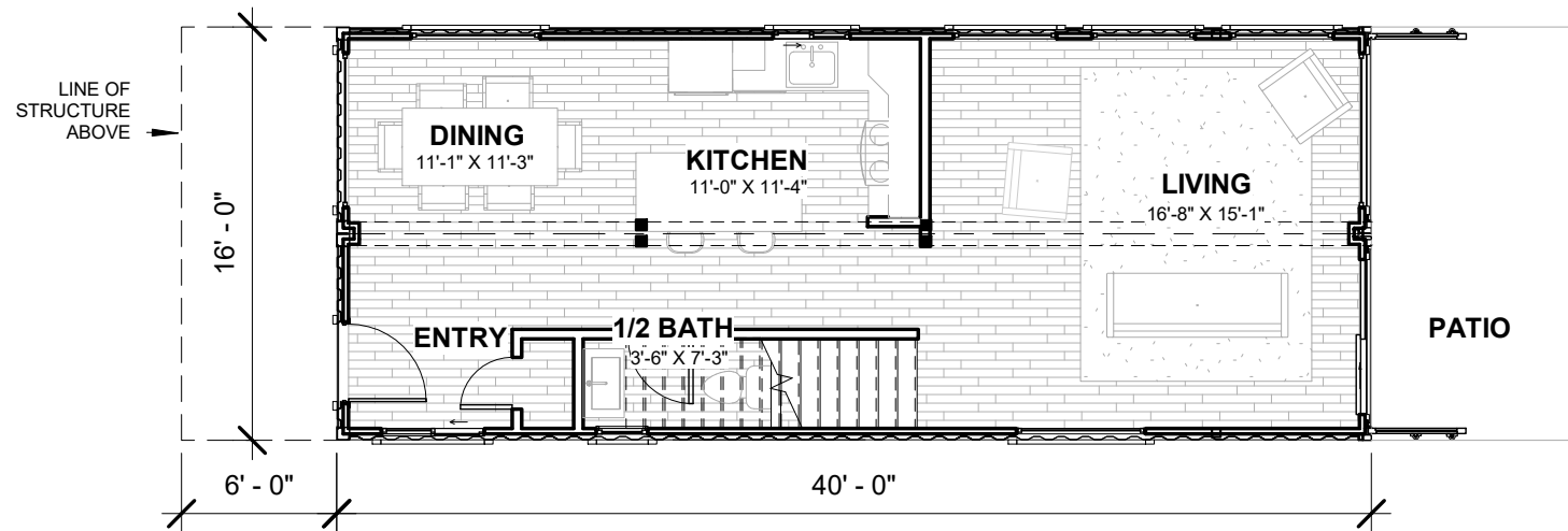
① LEVEL 1 1/8" = 1'-0"
