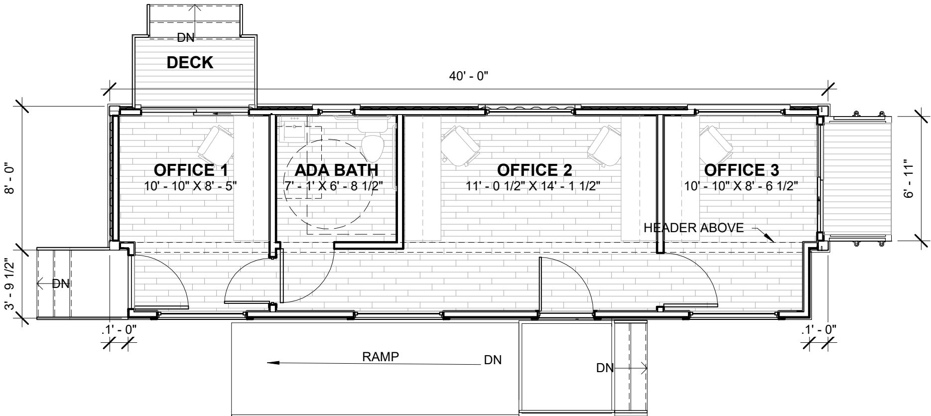
② FLOOR PLAN 3/16" = 1'-0"
