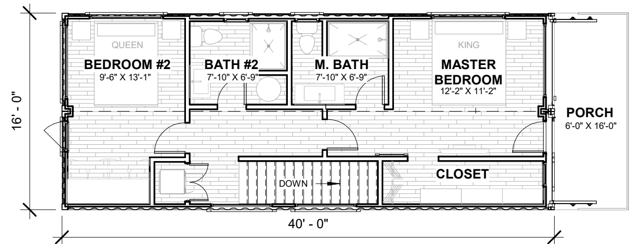
② LEVEL 2 MARKETING 1/8" = 1'-0"
