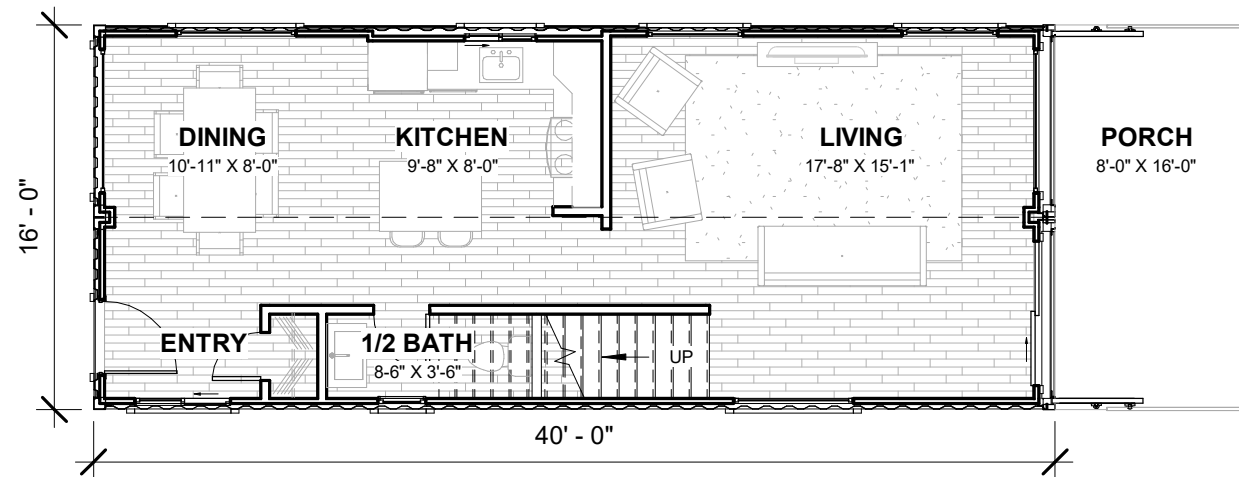
① LEVEL 1 MARKETING 1/8" = 1'-0"
