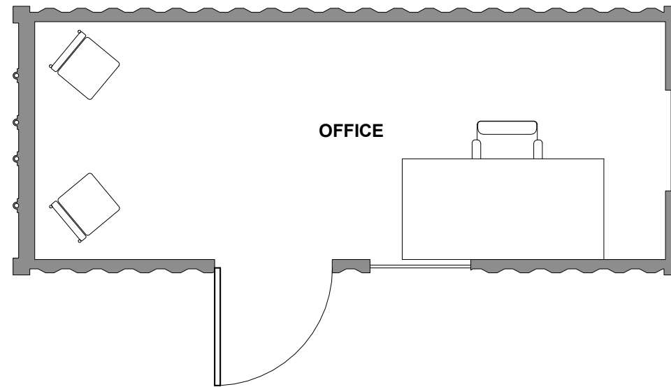
20' SINGLE OFFICE
