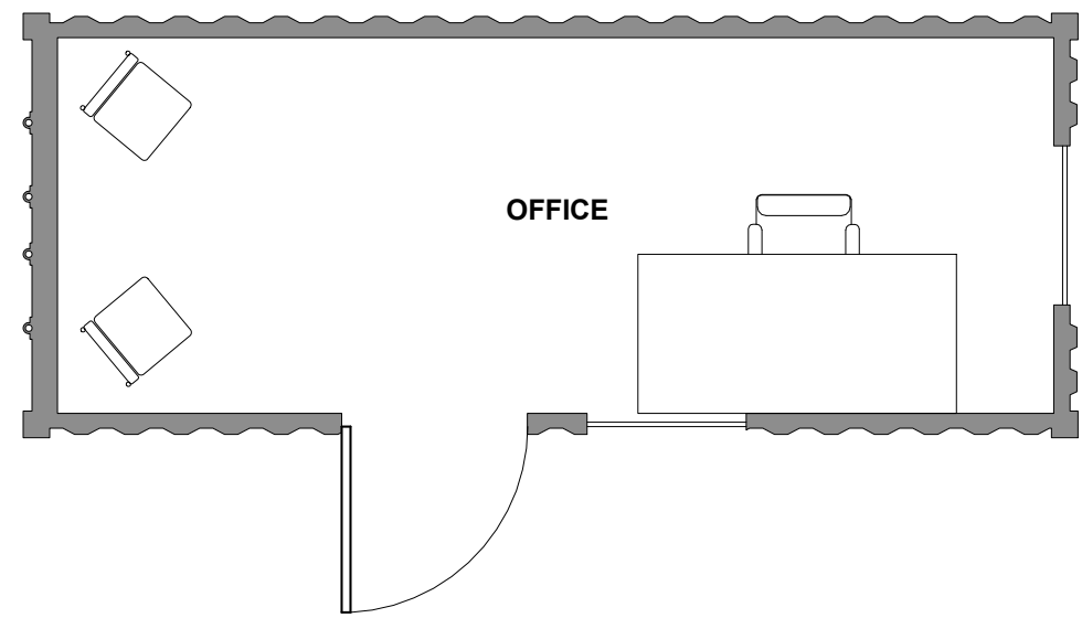
20' SINGLE OFFICE
