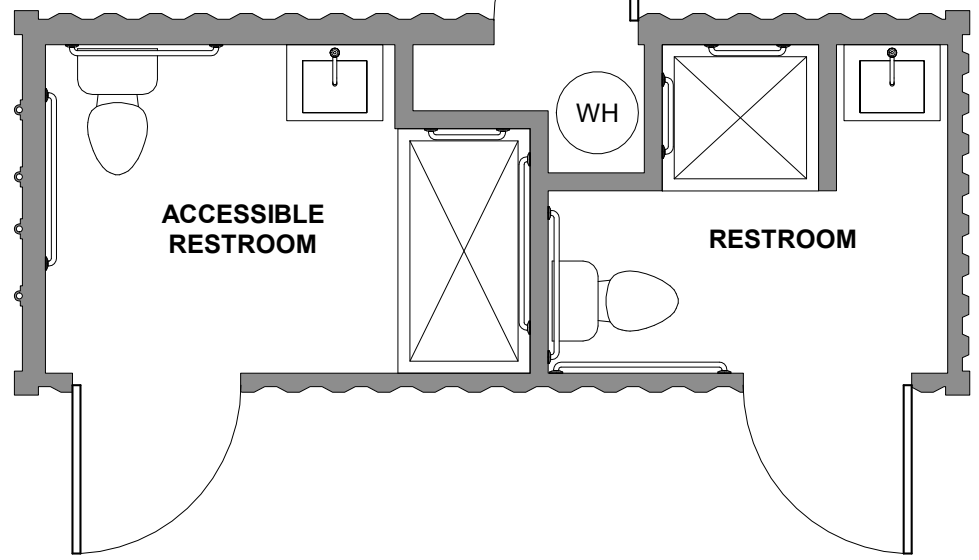
20' RESTROOM POD
